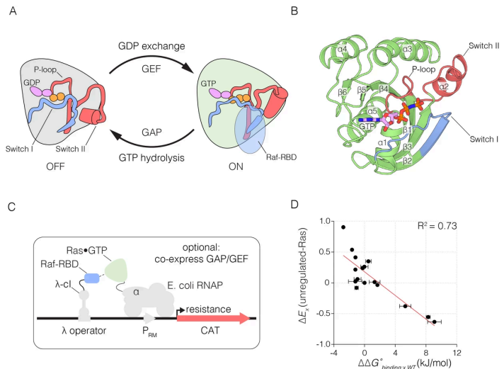
The Ras switching cycle and the bacterial two-hybrid system.
