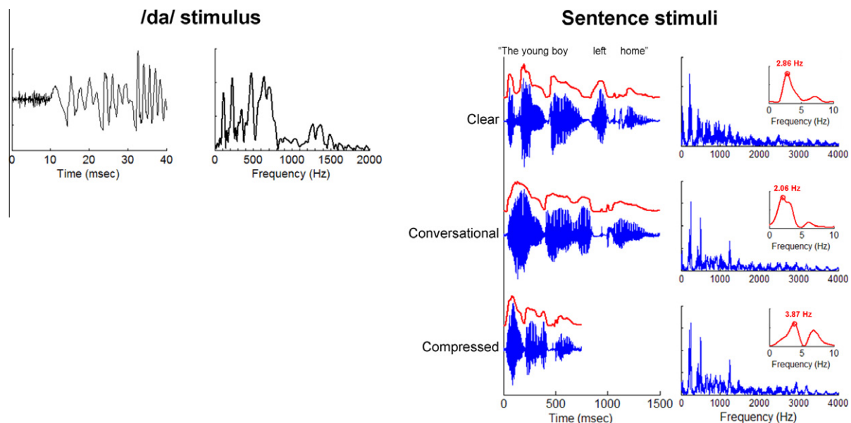
Fig. 2. Columns 1 and 2: brainstem stimulus “da” in the time and frequency domains. Column 3: cortical stimulus waveforms (blue) and broadband speech envelopes (red) for clear (top), conversational (center) and compressed (bottom) conditions. Greater amplitude envelope modulations are evident in the clear speech relative to the conversational stimuli. For example, there is no amplitude cue between “The” and “young” evident in the conversational stimulus envelope, however an amplitude cue is present in the clear stimulus envelope (0–450 ms post-stimulus onset). This phenomenon also occurs between the segments “boy” and “left” (450–900 ms post-stimulus onset). Column 4: frequency spectra for the three stimulus conditions (blue). Insets: frequency spectra of the speech envelopes (red) with the modal frequencies noted. (For interpretation of the references to color in this figure legend, the reader is referred to the web version of this article.)
