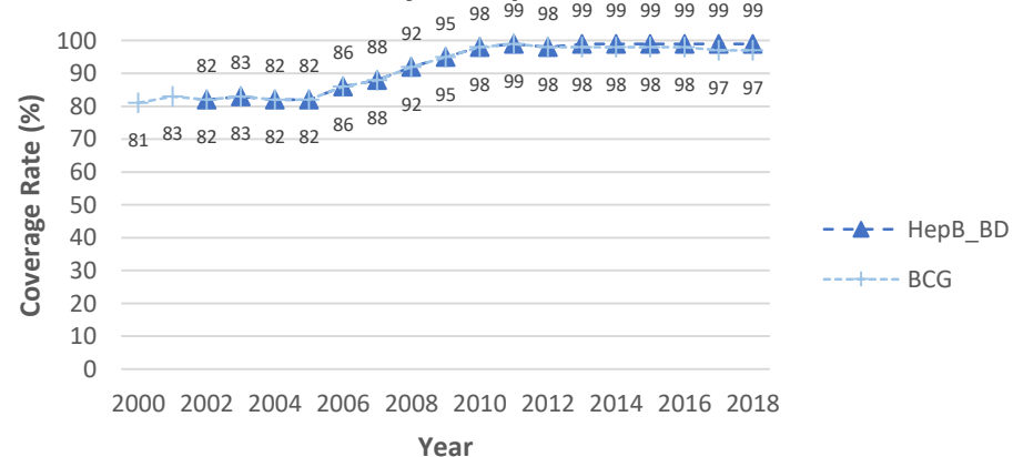
Azerbaijan: HepB BD vs. BCG
