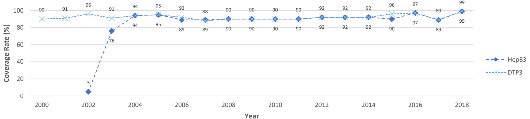
Trinidad and Tobago: HepB3 vs. DTP3
