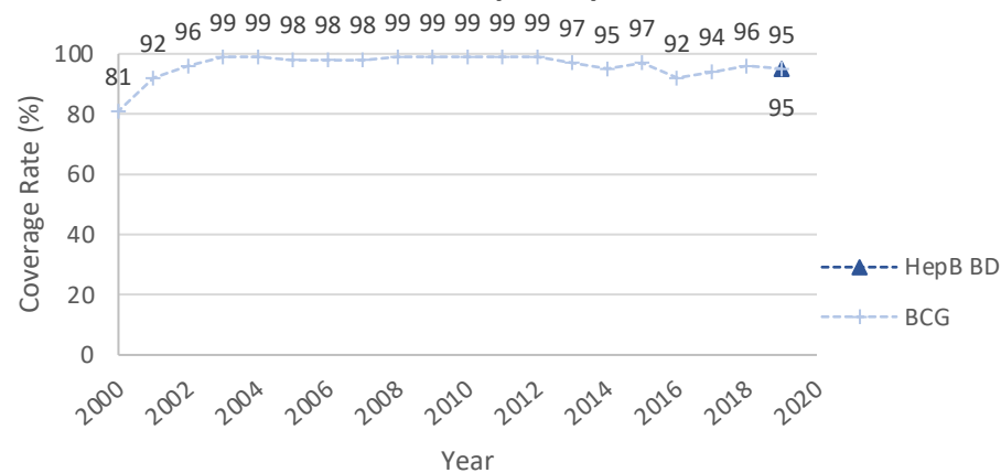
Sao Tome and Principe: HepB BD vs. BCG
