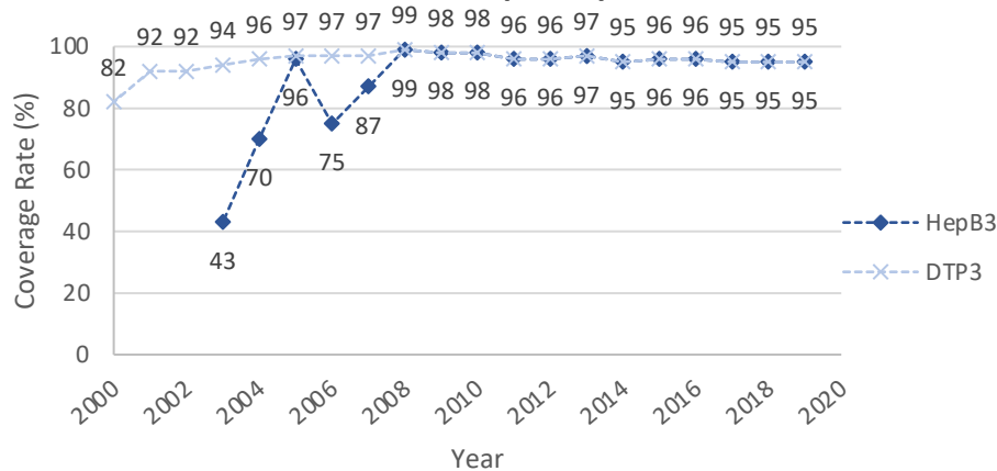
Sao Tome and Principe: HepB3 vs. DTP3
