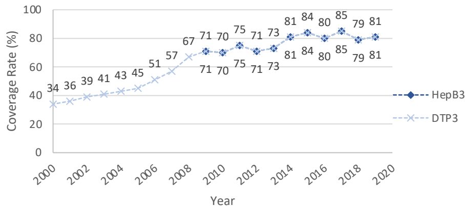
Niger: HepB3 vs. DTP3
