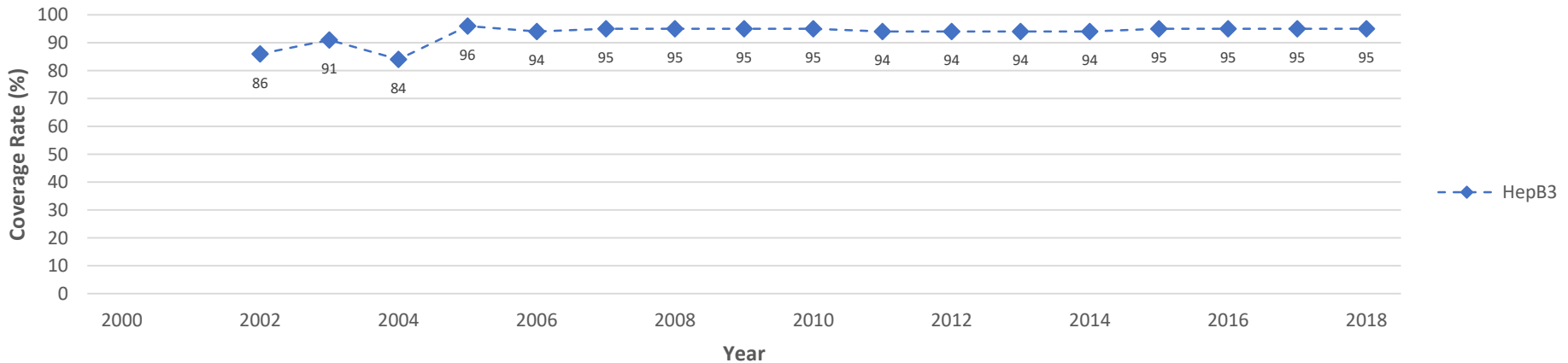
Eritrea: HepB3
