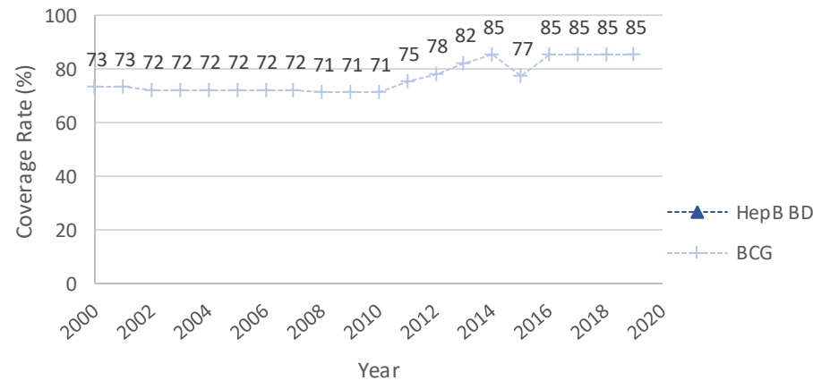
Equatorial Guinea: BCG
