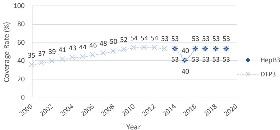
Equatorial Guinea: HepB3 vs. DTP3
