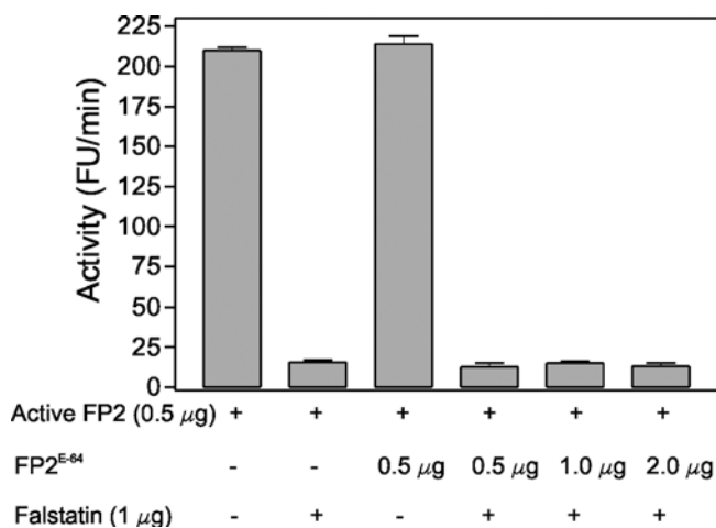
Figure 4. Mechanism of Interaction of Falstatin with Falcipain-2 Activity (arbitrary fluorescent units (FU) per minute) against Z-Leu-Arg-AMC is shown for indicated mixtures of falcipain-2 (FP2) and inactivated falcipain-2 (FP2 E64 ) with falstatin. Reaction components were incubated for 15 min before the addition of substrate and measurement of fluorescence over time. Error bars represent the standard deviations of results from two different assays, each performed in duplicate. doi:10.1371/journal.ppat.0020117.g004
