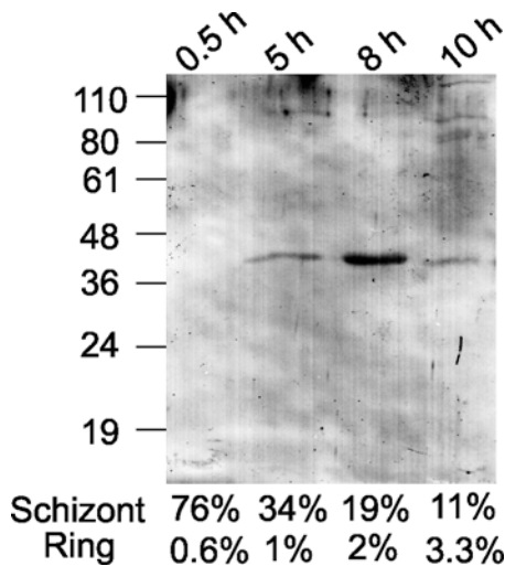
Figure 7. Release of Falstatin with Schizont Lysis
