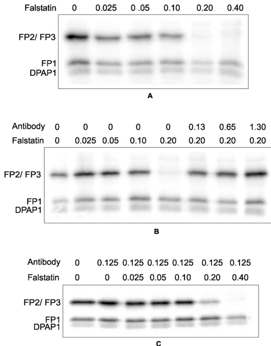
Figure 8. Inhibitor Competition
