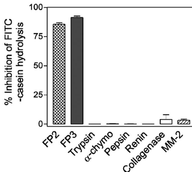
Figure 3. Activity of Falstatin against Different Classes of Proteases Equal amounts (4 \mu g) of proteases (FP2, falcipain-2; FP3, falcipain-3; trypsin; \alpha -chymo, \alpha -chymotrypsin; pepsin; renin; collagenase; MM-2, matrix-metalloprotease-2) were mixed with 350 \mu l of appropriate buffers containing falstatin (1.5 \mu g) for 15 min, FITC-casein (20 \mu g) was added, and hydrolysis of the substrate with and without falstatin was compared for each protease. Error bars represent the standard deviations of results from two different assays, each performed in duplicate. doi:10.1371/journal.ppat.0020117.g003
