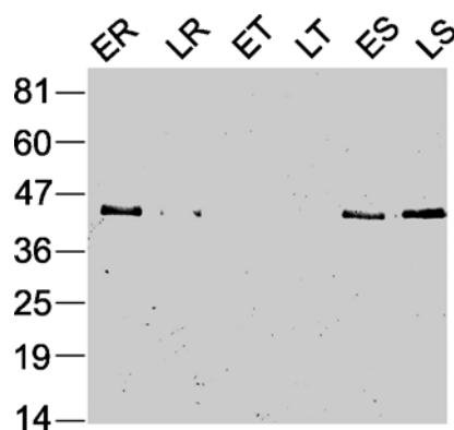
Figure 5. Stage-Specific Expression of Falstatin Extracts from highly synchronized parasites were collected every 8 h, separated by SDS-PAGE, and evaluated by immunoblotting with anti-falstatin antibodies. Each sample of early-ring, late-ring, early-trophozoite, late-trophozoite, early-schizont, or late-schizont extracts corresponded to 1.3 \times 10^7 parasitized cells. The positions of molecular weight markers (kDa) are indicated. ER, early-ring; LR, late-ring; ET, early-trophozoite; LT, late-trophozoite; ES, early-schizont; LS, late-schizont. doi:10.1371/journal.ppat.0020117.g005
