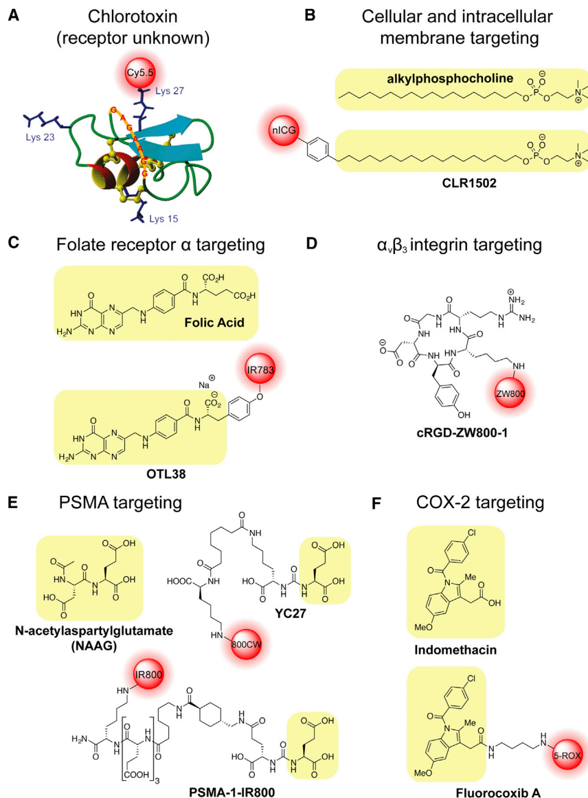
Figure 3. Affinity-Based Probes
