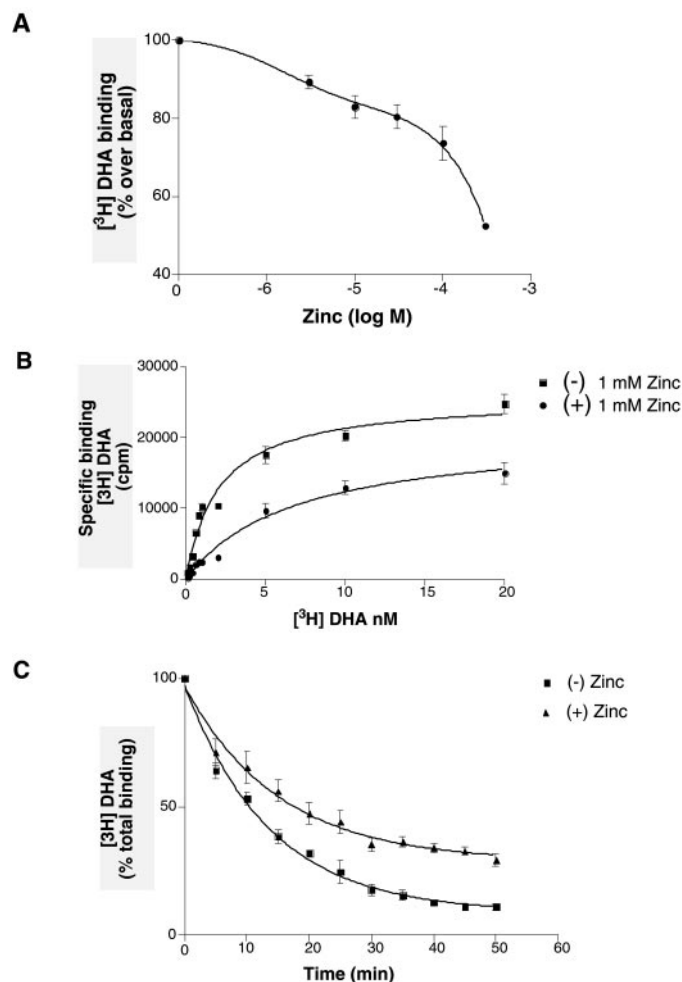
Fig. 1. Effect of zinc on antagonist binding in membranes expressing \beta_2 AR. A, inhibition of [^3\text{H}]\text{DHA} binding to \beta_2 AR by zinc. Sf9 membranes expressing \beta_2 AR ( 15.2 \text{ pmol/mg} ) were incubated with different concentrations of zinc in the presence of 1 \text{ nM } [^3\text{H}]\text{DHA} . The DHA binding in the absence of zinc is referred to as basal binding and was set to 100%. Maximum inhibition of antagonist binding was around 1 \text{ mM } Zn^{2+} . B, saturation binding of [^3\text{H}]\text{DHA} ( 100 \text{ pM} – 20 \text{ nM} ) on membranes expressing \beta_2 AR ( 8.7 \text{ pmol/mg} ) in the presence and absence of 1 \text{ mM } Zn^{2+} . Zn^{2+} caused an increase of nearly 3-fold in apparent K_D value for DHA ( 1.489 \pm 0.23 \text{ nM} control, 4.877 \pm 1.178 \text{ nM} with Zn^{2+} ) and \sim 40\% decrease in B_{\text{max}} value. Data were best fit to monophasic saturation hyperbolae. These data are representative of three different experiments done in triplicate. C, effect of zinc on the rate of antagonist dissociation from \beta_2 AR. Dissociation rate kinetics measured for [^3\text{H}]\text{DHA} binding to membranes expressing \beta_2 AR ( 7 \text{ pmol/mg} ) was determined in the presence (triangles) or absence (squares) of 1 \text{ mM } Zn^{2+} as described under Experimental Procedures . Data shown are the mean \pm S.D. of three independent experiments performed in triplicate.
