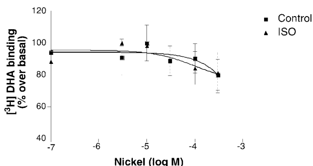
Fig. 7. Effect of divalent ions on the agonist affinity. The effect of \text{Co}^{2+} (A) and \text{Ni}^{2+} (B) on [^3\text{H}]\text{DHA} binding in presence and absence of 100 nM isoproterenol was determined using Sf9 membranes expressing \beta_2\text{AR} (7 pmol/mg). Assay mixtures contained \sim 25 \mu\text{g} of membrane protein, 1 nM [^3\text{H}]\text{DHA} , and 10 \mu\text{M} \text{GTP}\gamma\text{S} . Nonspecific binding was less than 10% of total binding. Data represent the mean \pm S.D. of three independent experiments. Each of these experiments was performed in triplicate. Binding data were analyzed for best fit to two affinity states.
