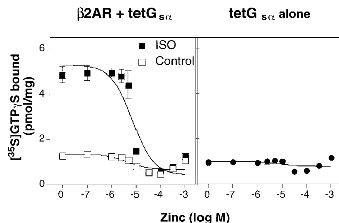
Fig. 8. Effect of \text{Zn}^{2+} on [^{35}\text{S}]\text{GTP}\gamma\text{S} binding in Sf9 membranes coexpressing \beta_2\text{AR} (12.7 pmol/mg) and \text{tetG}_{\text{s}\alpha} . \text{GTP}\gamma\text{S} binding was done on Sf9 membranes in presence of different concentrations of zinc. (—) Iso-proterenol (10 \mu\text{M} ) was used as agonist. \text{Zn}^{2+} inhibits receptor-stimulated \text{GTP}\gamma\text{S} binding to \text{tetG}_{\text{s}\alpha} ( \text{IC}_{50} of 7.2 \mu\text{M} ) (left). The effect of \text{Zn}^{2+} on \text{GTP}\gamma\text{S} binding to membranes expressing \text{tetG}_{\text{s}\alpha} alone (right).
