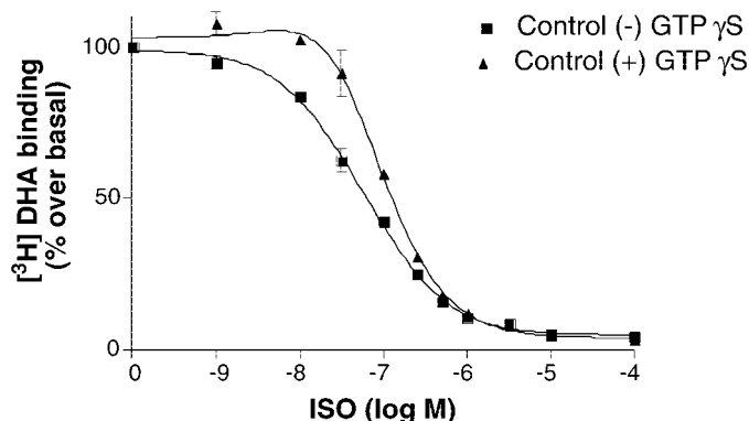
Fig. 3. Effect of GTP \gamma S on isoproterenol competition of DHA binding to Sf9 membranes expressing \beta_2AR together with tet G_{s\alpha} . Isoproterenol competition in presence and absence of unlabeled GTP \gamma S (10 \mu M ) was performed as described under Experimental Procedures . Reaction mixtures contained 10 \mu g of protein/tube. The membranes expressing the protein were 15.7 pmol/mg. Data shown are the mean \pm S.D. of three independent experiments performed in triplicate. Binding data were analyzed for best fit to two affinity states.
