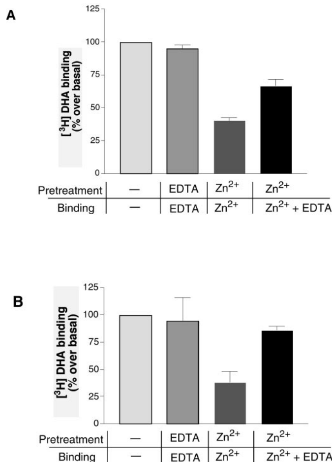
Fig. 2. Reversibility of the Zn^{2+} effect on antagonist binding. Membrane-bound (A) or purified \beta_2 AR (B) was preincubated with either 1 \text{ mM } ZnCl_2 , 5 \text{ mM} EDTA, or nothing for 30 \text{ min} on ice. After the pretreatment period, radioligand ( 2 \text{ nM } [^3\text{H}]\text{DHA} ) and either 5 \text{ mM} EDTA or nothing was added and incubated for 1 \text{ h} at room temperature. The membranes were then harvested by rapid filtration and soluble receptor was harvested by gel filtration as described under Experimental Procedures . Data shown are the mean \pm S.D. of three independent experiments performed either in duplicate for purified protein or triplicate for membranes.
