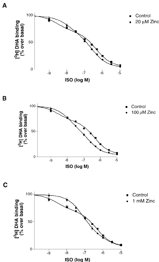
Fig. 4. Modulation of agonist binding by Zn^{2+} . A to C, isoproterenol competition binding was performed on membranes expressing \beta_2AR (12.7 pmol/mg) together with tet G_{s\alpha} in the presence of 20 \mu M Zn^{2+} (A), 100 \mu M Zn^{2+} (B), and 1 mM Zn^{2+} (C). The antagonist binding observed in the absence of any competitor was set to 100%. In A to C, binding in the absence of Zn^{2+} is shown for reference. In the presence of 20 to 100 \mu M Zn^{2+} , GTP \gamma S-sensitive high-affinity binding is lost, yet the affinity of the low-affinity binding is increased. Reaction mixtures contained 1 nM [ ^3H ]DHA and isoproterenol at the indicated concentrations. Binding data were analyzed for best fit to two affinity states. Data represent the mean of three independent experiments. Each experiment was performed in triplicate.
